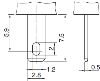
Solder/Tab Terminal
