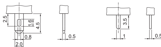
Soldering Terminal
